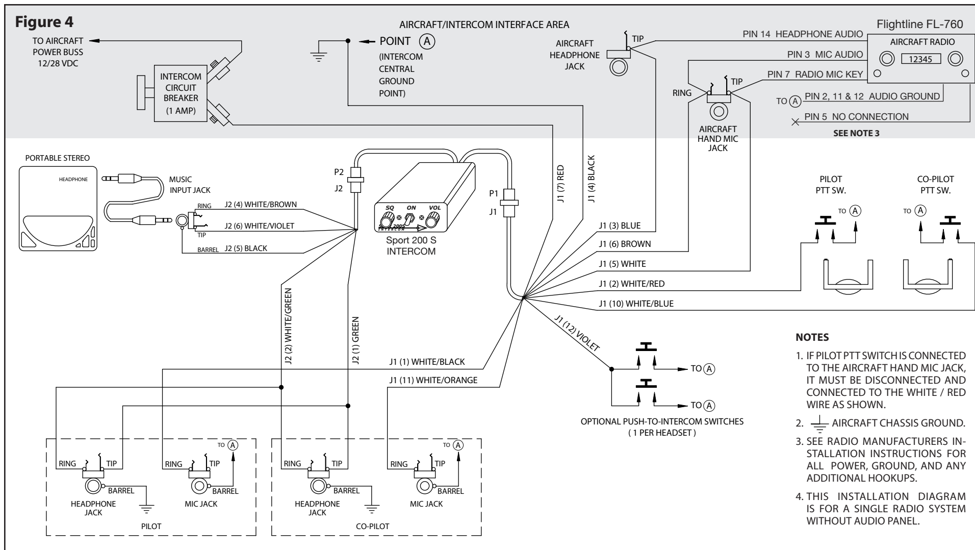
Sport 200S – Flightline FL-760 Radio Installation Wiring Diagram
